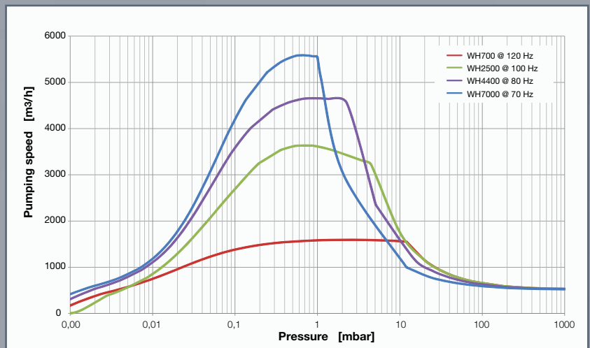
Pumping speed of RUVAC WH in combination with DRYVAC DV650 S
